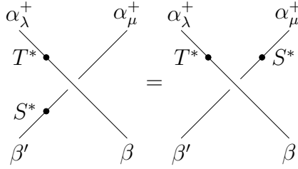
Figure 10: A naturality equation
